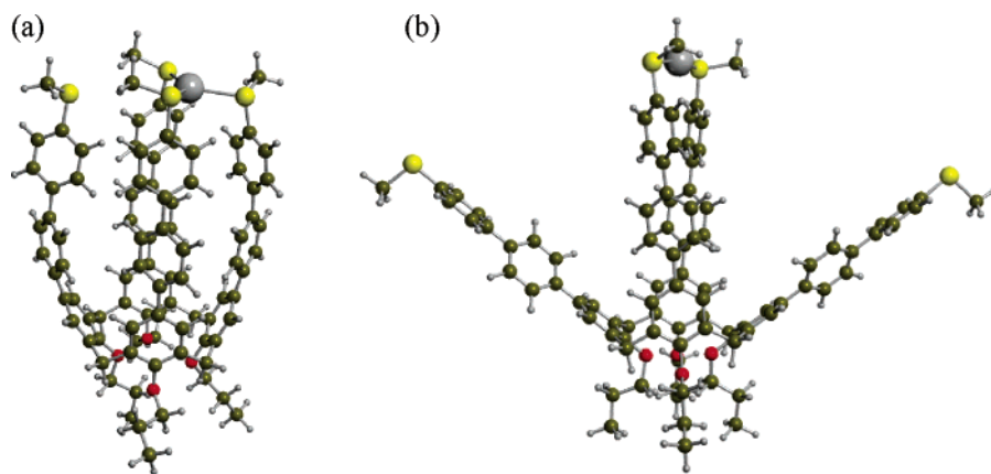
FIGURE 2. DFT-optimized geometries of an analogue of 4\mathbf{a}\cdot\text{Ag}^+ complex for the (a) pseudo- C_{4v} binding mode and (b) near the C_{2v} binding mode. The drawings were performed by MOLDRAW. 19
